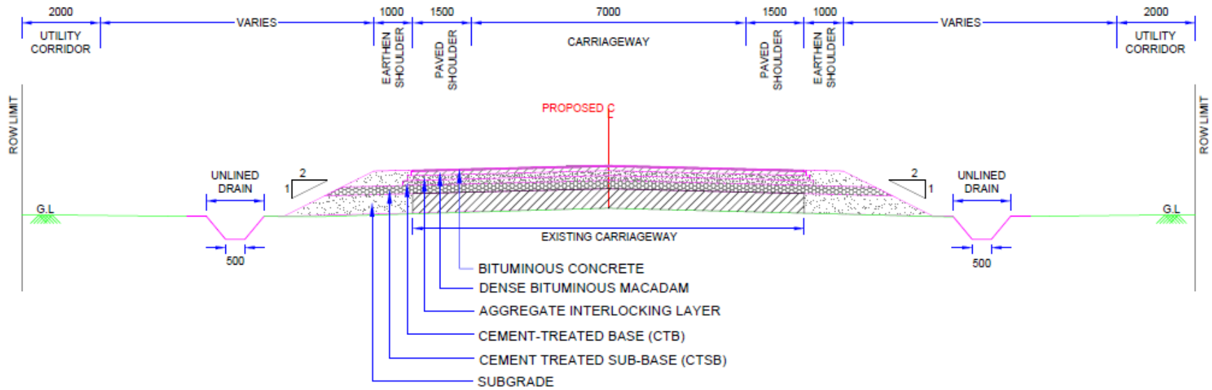
TCS-XI: 2 LANE CARRIAGEWAY
