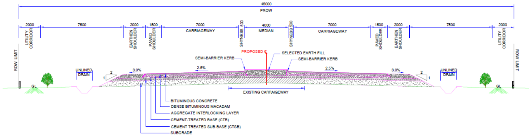
TCS-IA: 4 LANE DIVIDED CARRIAGEWAY CONCENTRIC WIDENING
