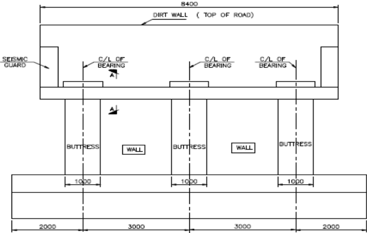
LONGITUDINAL ELEVATION OF SUB-STRUCTURE
