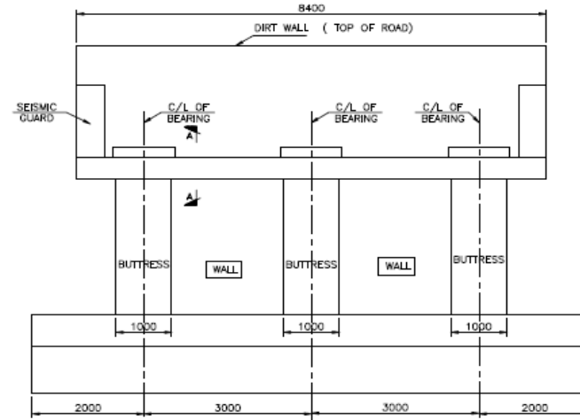
LONGITUDINAL ELEVATION OF SUB-STRUCTURE
