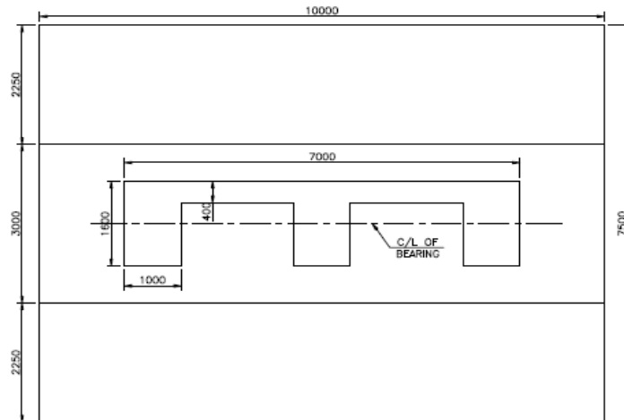
PLAN OF FOUNDATION
