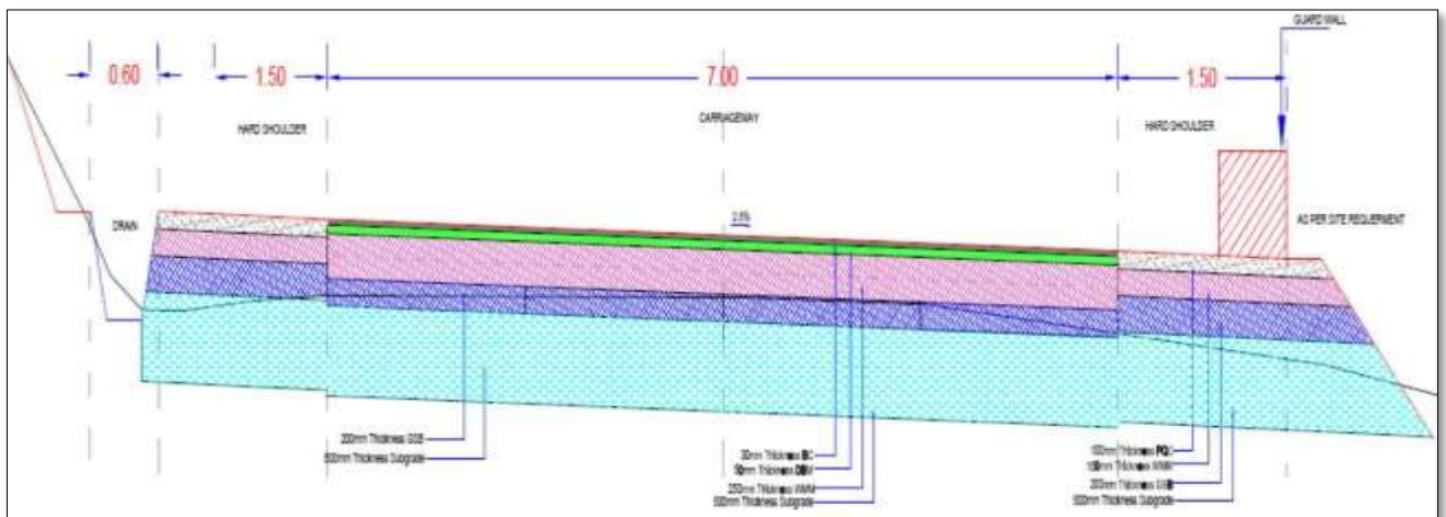
Figure 3: Typical Cross Section III in Open Section
