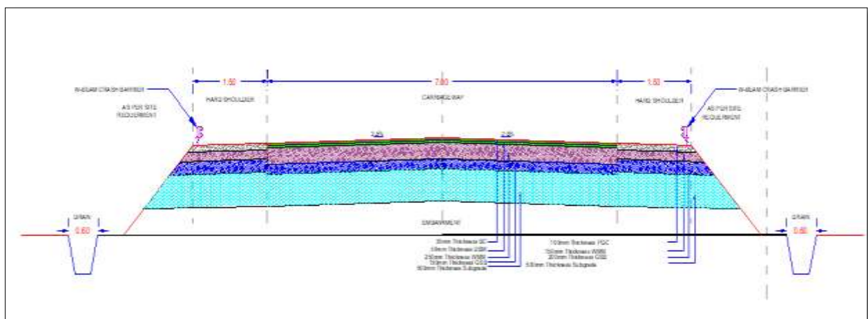
Figure 3: Typical Cross Section III in Open Section
