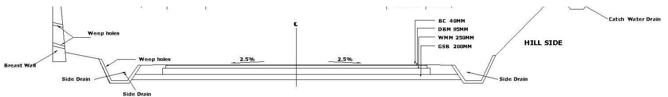
Fig - 2.14(new) (Hilly Terrain) Typical Cross Section 2-lane Carriageway (With Paved Shoulders) Box Cut With one side Breast Wall
