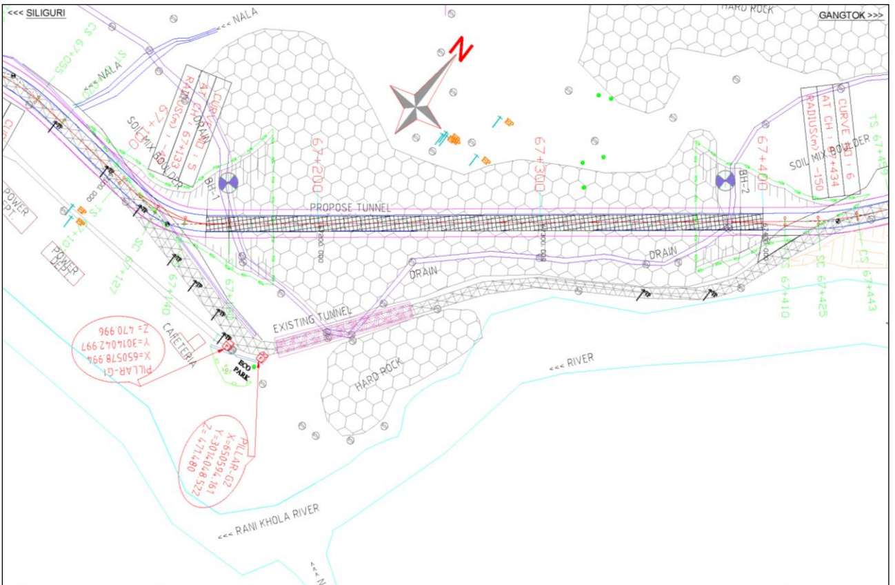
Site survey Map at proposed Tunnel Location
