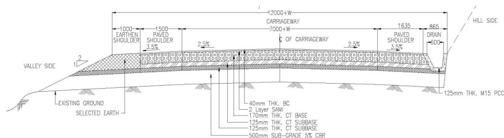
TYPICAL PAVEMENT DETAILS FOR MAIN ROAD
