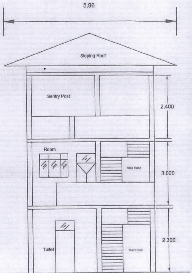
Front Elevation
