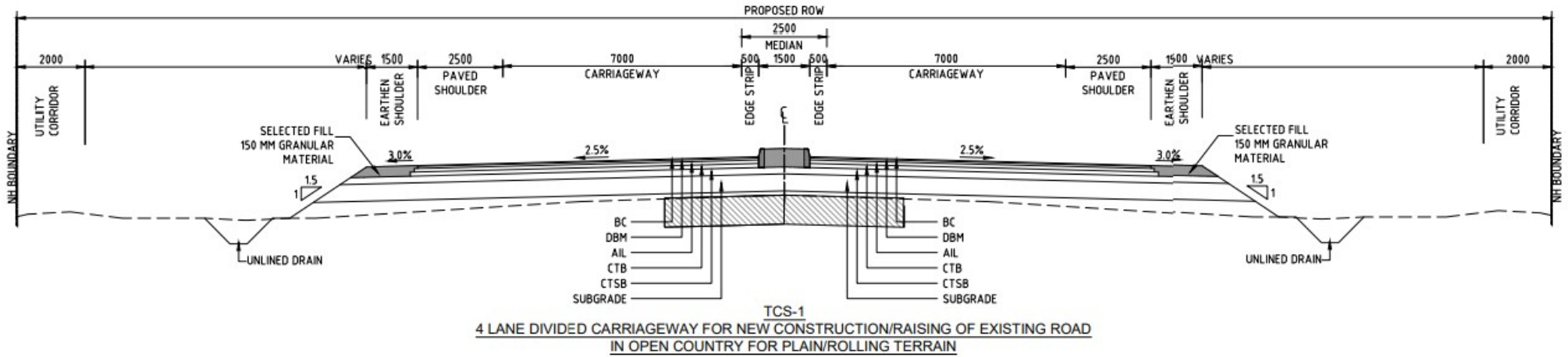
Figure of Typical Cross Section: -
