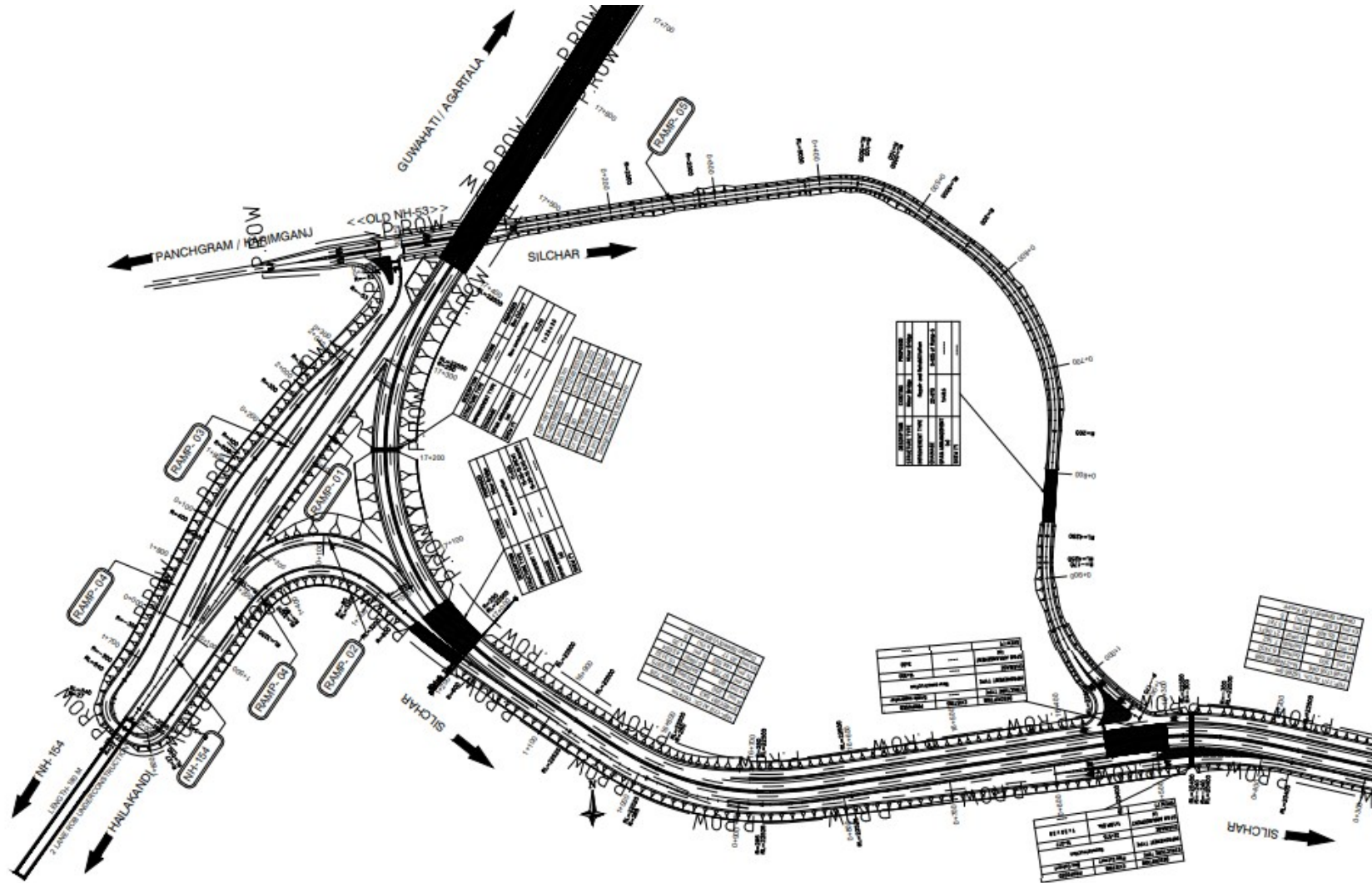
Layout Plan of Interchange near Km 16+284: -
