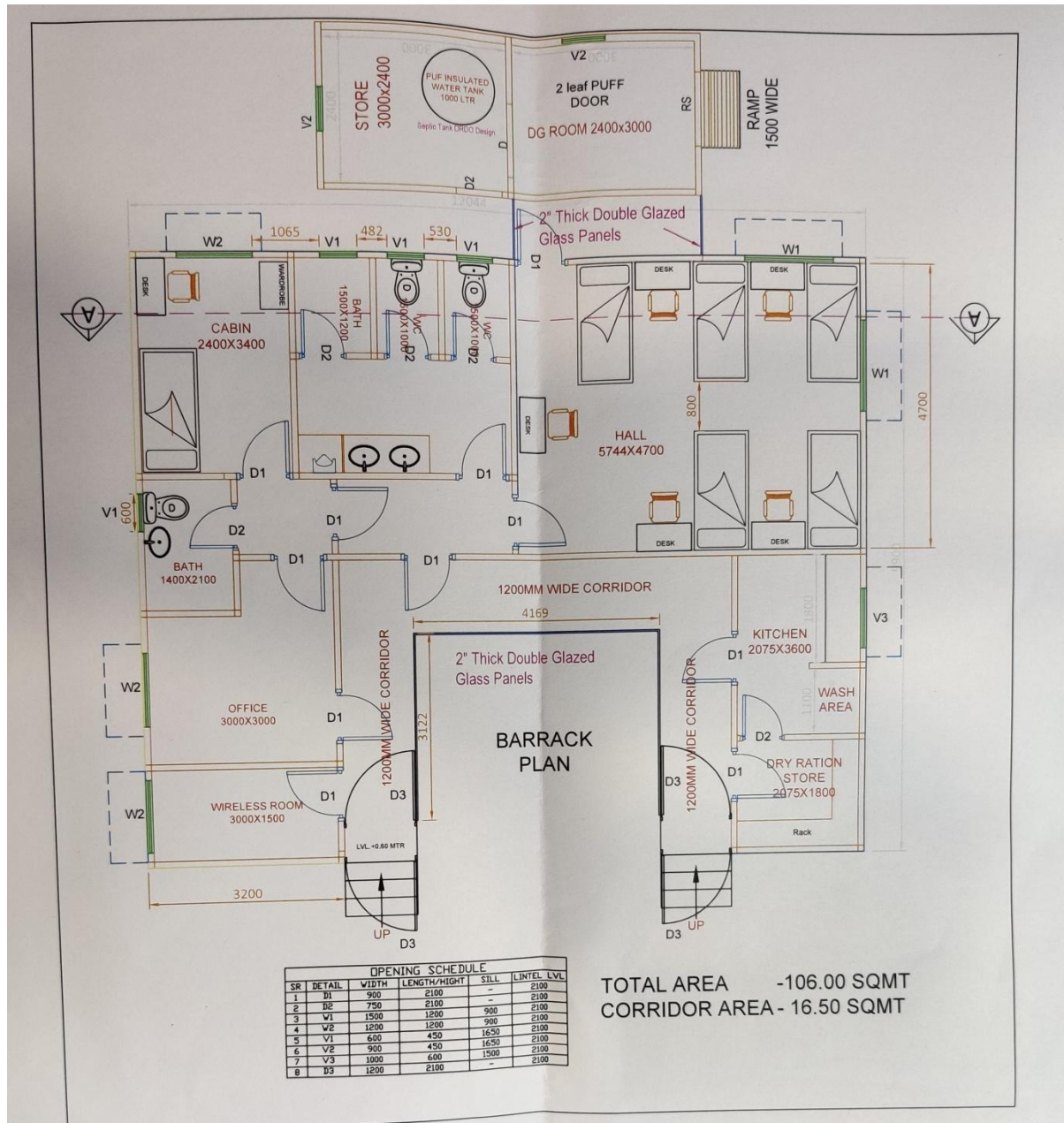
Plan for office cum residence including location of Water Tank, Septic Tank, Store & Gen-Set
