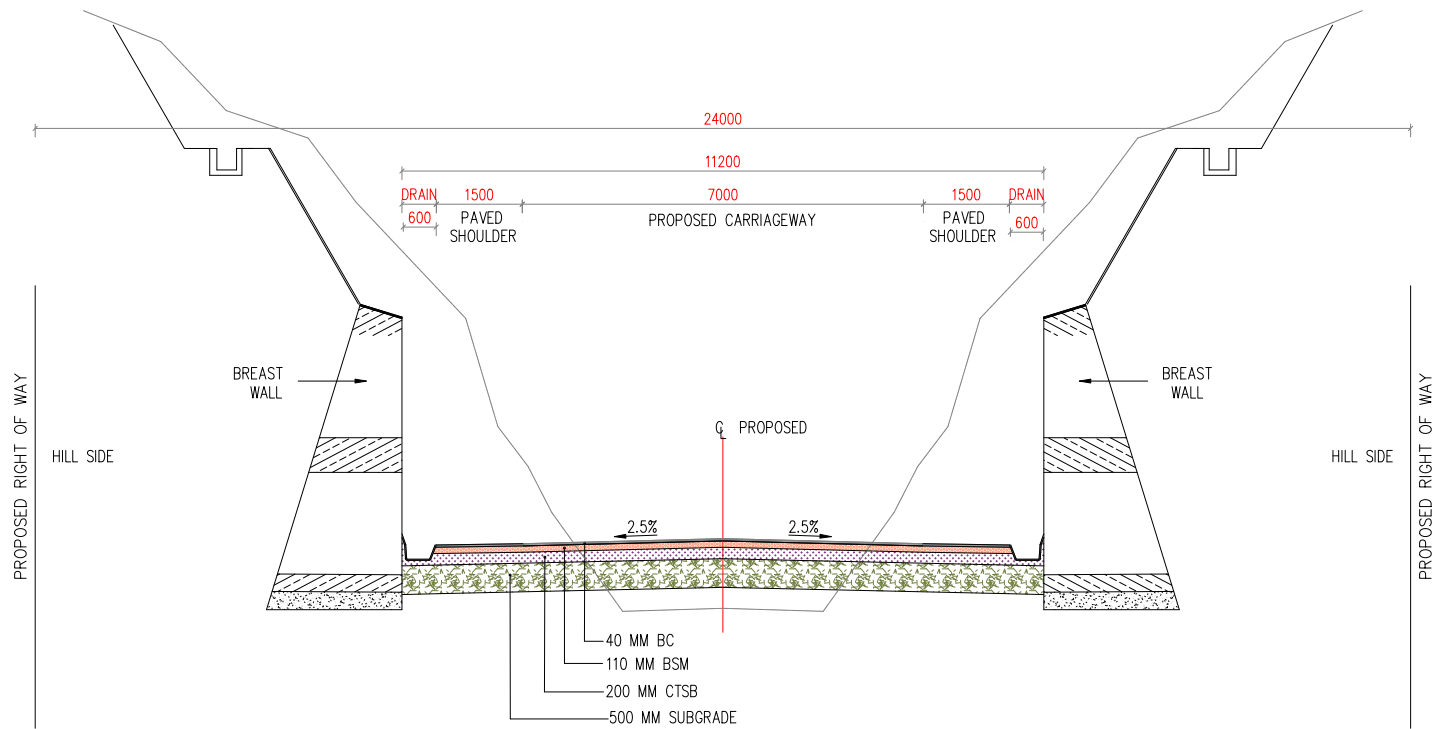
TCS-I Two Lane With Paved Shoulder New alignment (Both Side Hill Section)
