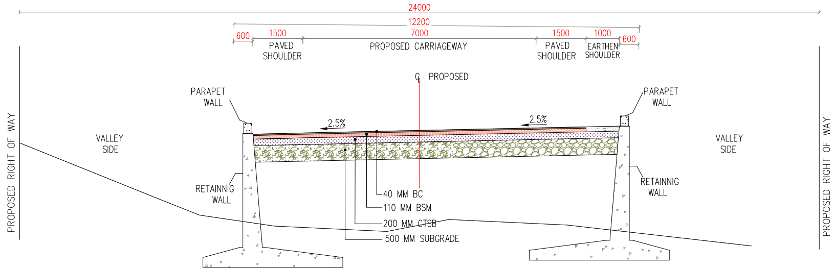
TCS-III Two Lane With Paved Shoulder (Both Side Valley Section) (New-Alignment)
