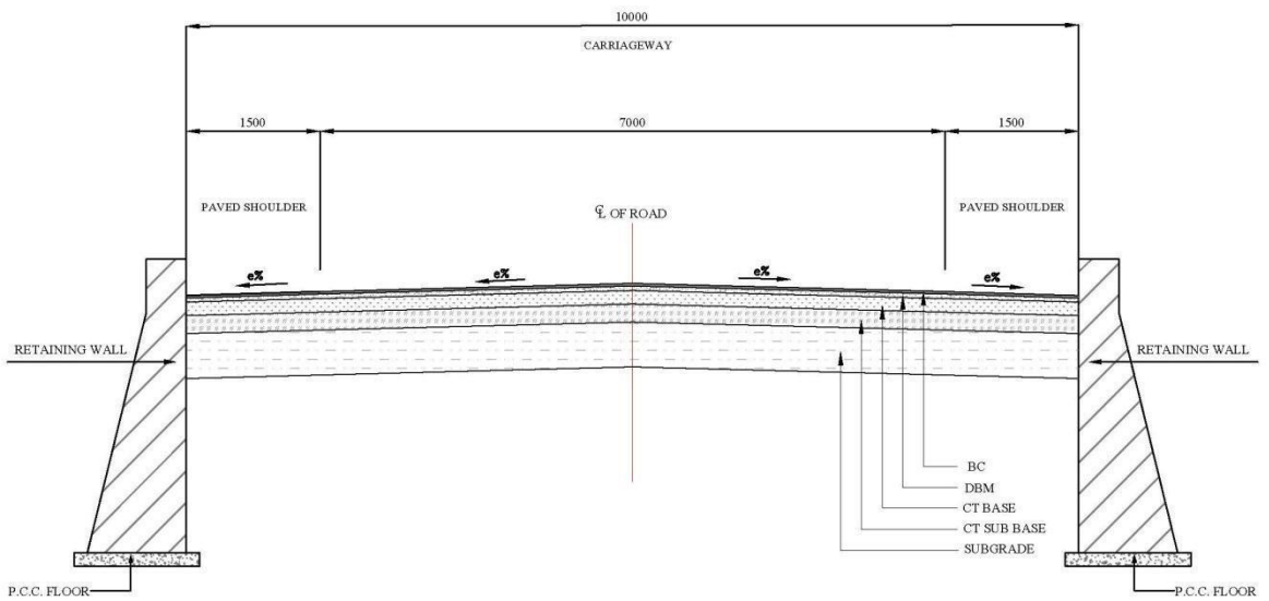
TYPE- 6 TWO LANE + PAVED SHOULDER (Both Side)RETAINING WALL
