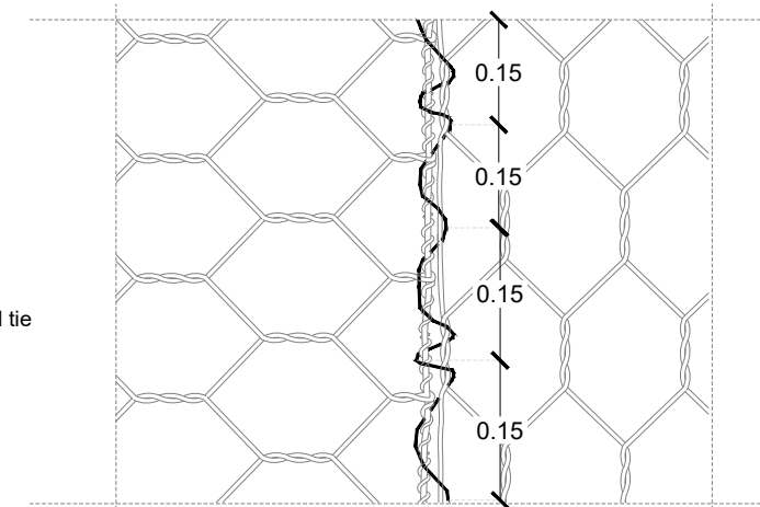
LACING DETAIL
